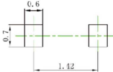
SOD-523F Pattern Recommendation
